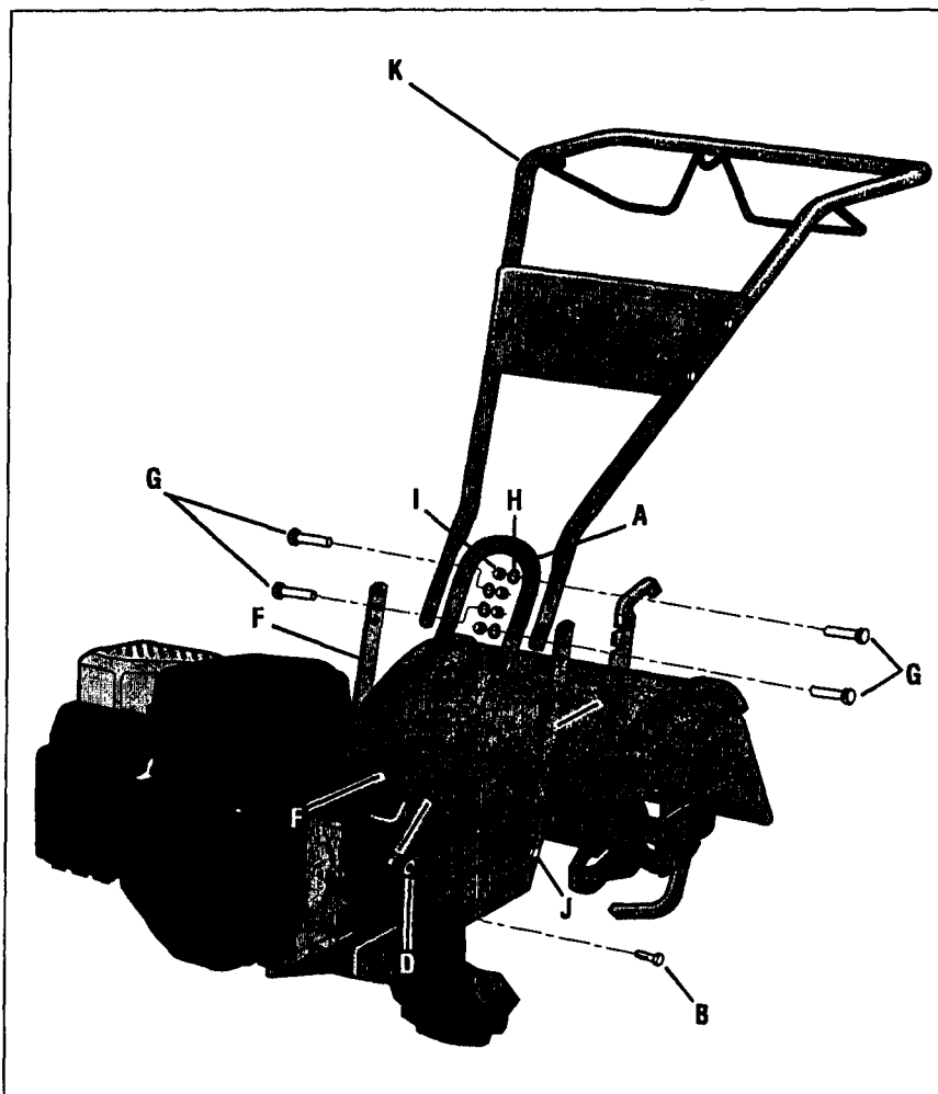
Illustration 2-2 : Attacher le guidon
